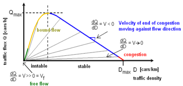
Fig. 1 Fundamental Diagram of Traffic Flow
